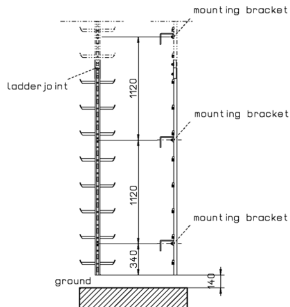
Fig. 2c Mounting distance: 1120 mm
