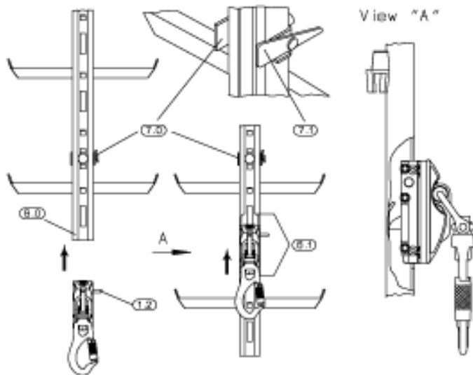
Fig. 2 - Illustration: self-locking carabiner hook
