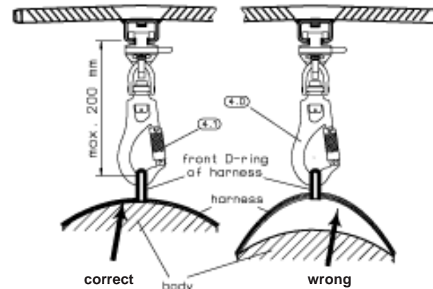
Fig. 3 - Illustration: self-locking carabiner hook
